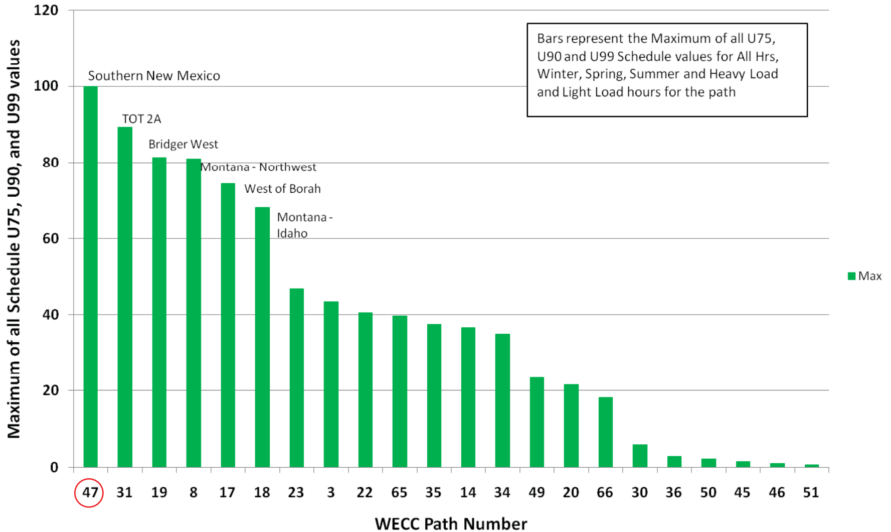
Figure IV-4 Path Congestion Ranking - SCHEDULES - Ranking Method #4 Ranking based upon the Path Maximum of all Path Schedule Metrics Nov 1, 2006 thru Oct 31, 2007
