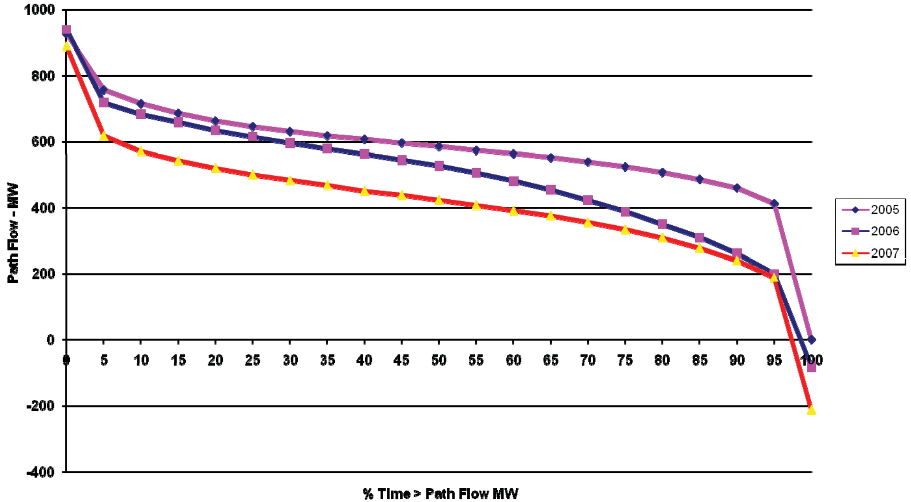
Figure II-42 Southern New Mexico - Path 47 Actual Path Flow 2005, 2006 and 2007
