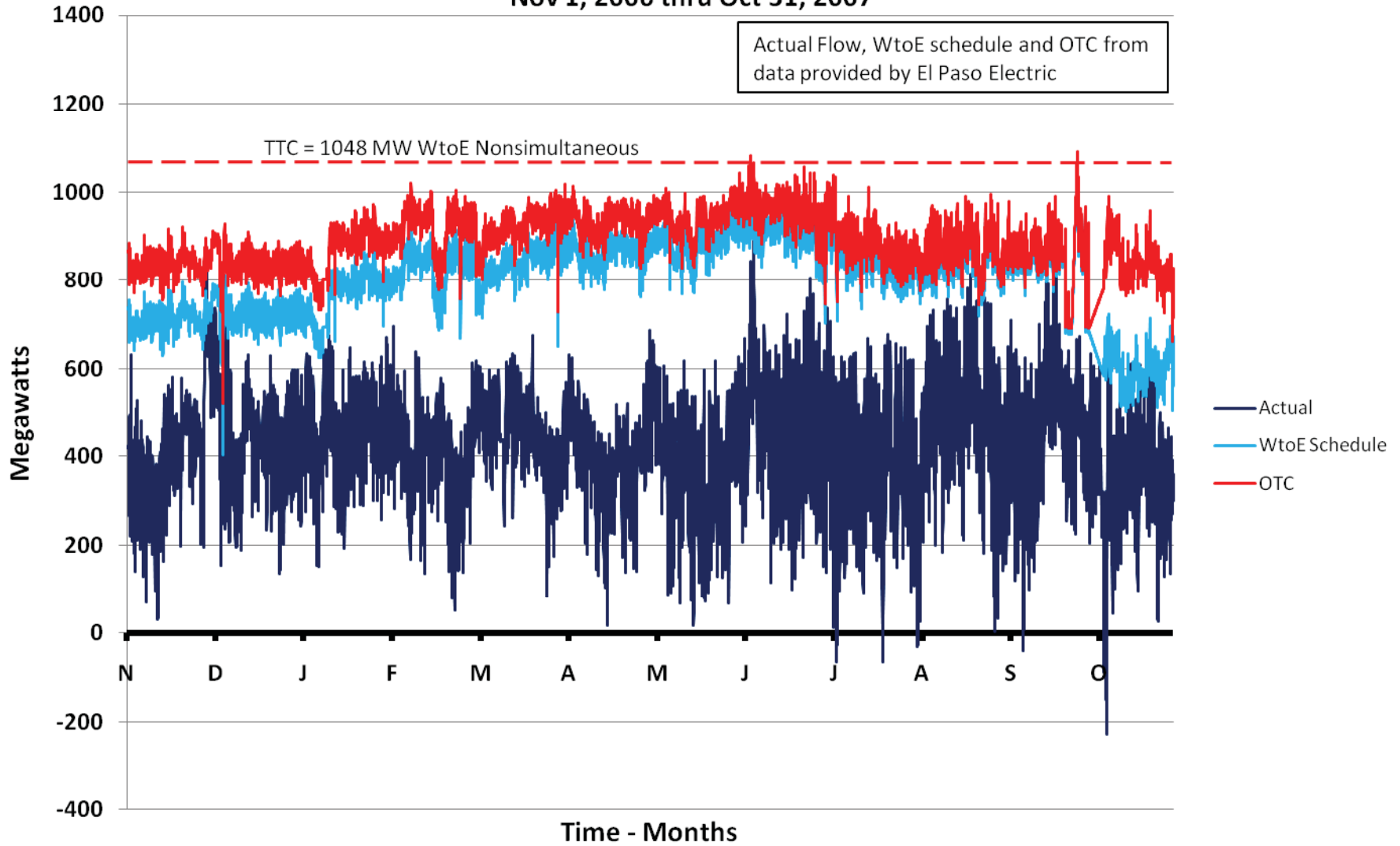
Figure II-40 Southern New Mexico - Path 47 Actual Flow and Inbound Schedule (F+NF) - from El Paso Electric data Nov 1, 2006 thru Oct 31, 2007
