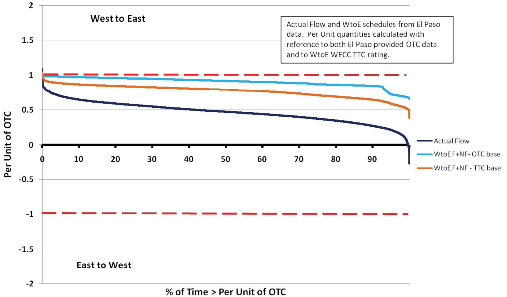
Figure II-41 Southern New Mexico - Path 47 Actual Flow and WtoE Schedule Nov 1, 2006 thru Oct 31, 2007
