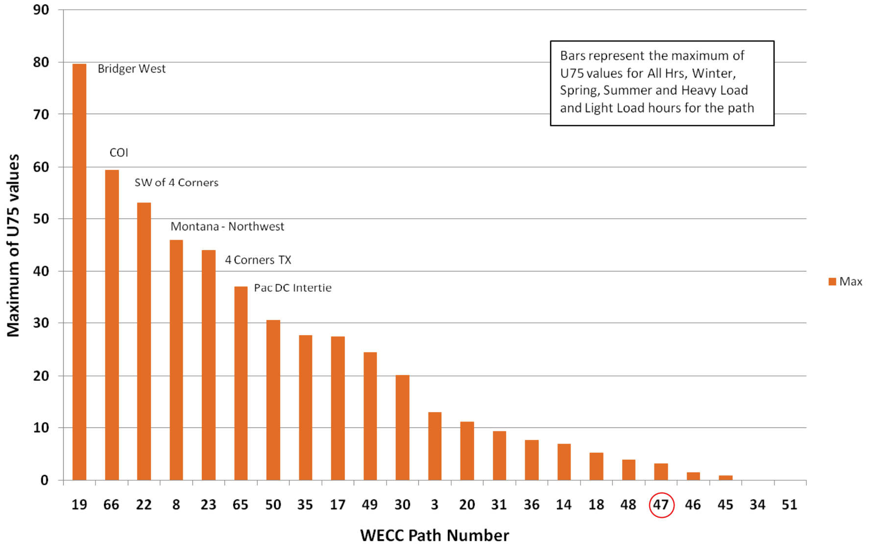
Figure IV-2 Path Congestion Ranking - ACTUAL FLOW - Ranking Method #2 Nov 1, 2006 thru Oct 31, 2007
