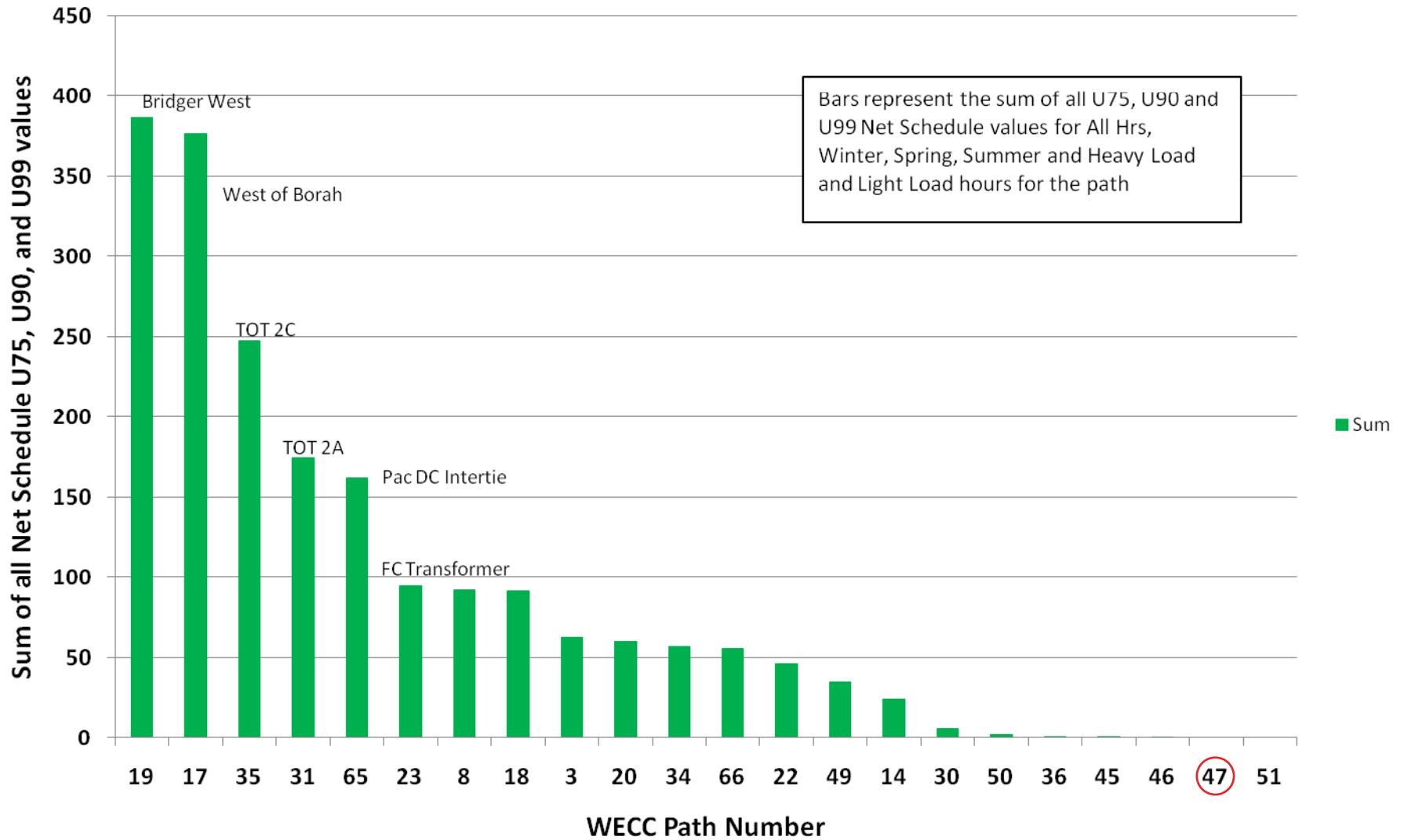
Figure IV-3 Path Congestion Ranking - SCHEDULES - Ranking Method #3 Ranking based upon the Sum of all NET Schedule Metrics Nov 1, 2006 thru Oct 31, 2007
